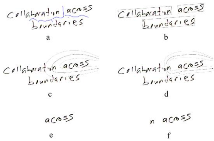
Fig. 3.15 Steps in the sloppy selection gesture interpretation technique. a, b Detection of word objects. c, d , Inference of gesture carefulness vs. sloppiness. e, f Decision whether to select based on word groups or precise gesture path
