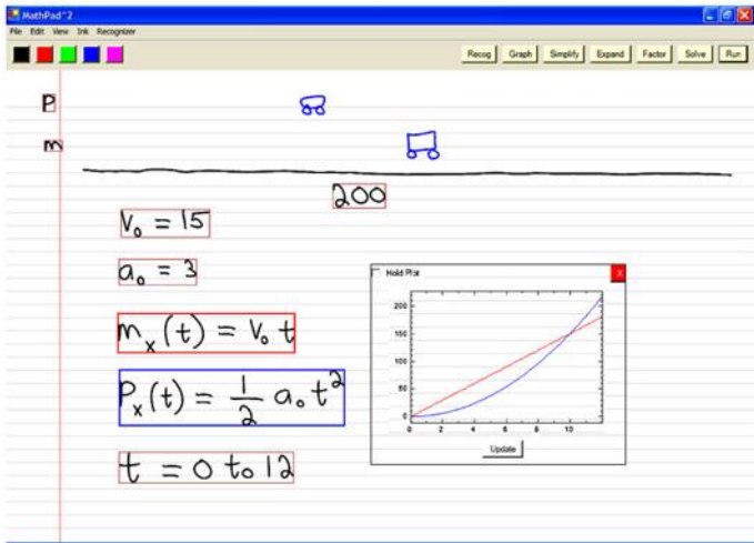
Fig. 4.4 The MathPad 2 prototype. The mathematical sketch shows two cars moving down a road, one with constant velocity and one with constant acceleration. The user writes down the mathematics, draws a road and two cars, and associates the mathematics to the drawing using labels. Running the sketch animates the two cars, illuminating how a car moving with constant acceleration will overtake the car with constant velocity. The sketch also shows a graph of the two equations of motion
