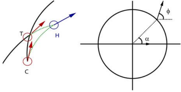
Fig. 12.11 (Left) Given a tee point T , a cusp C and tangent vectors at these points, we need to estimate the hidden cusp H and the tangent vector at H . (Right) Precomputing the table of hidden-cusp locations for a number of sampled locations and directions
