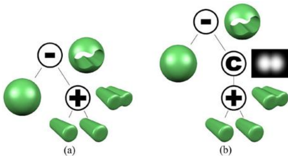
Fig. 11.19 In (a), two cylinder primitives are blended, and then subtracted from a sphere. In (b), a cache node is inserted above the blend node. Once filled, the cache short-circuits evaluation of the blend subtree, replacing an O(m) traversal with an O(1) tri-linear interpolation
