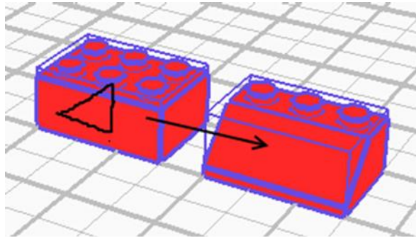
Fig. 7.21 Inserting a part by sketching its width and length. Here, the system suggests a brick that satisfies these dimensions. Other possibilities are presented in the suggestion list
