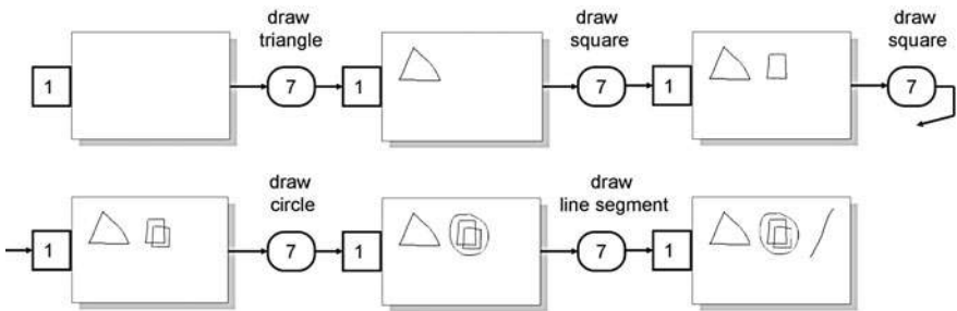
Fig. 3.9 Steps of the interaction flow for Task I under the Interaction Flow protocol of a conventional Electronic Whiteboard program. Numbers indicate nodes of the Interaction Flow Diagram of Fig. 3.8
