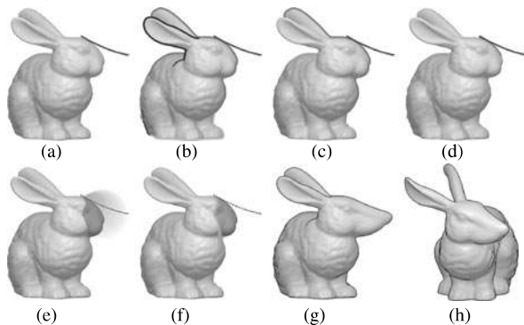
Fig. 9.19 Algorithm pipeline. Top row , from left to right: a user sketch, b image-space silhouettes, c retained silhouettes after proximity culling, d handle estimation; Bottom row , left to right: e correspondences and ROI estimation by bounding volumes, f setup for Laplacian Surface Editing, g and h deformation result. Note that the user only sees a , g and h
