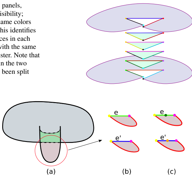
Fig. 12.22 a A contour-completed drawing of a leg attached to a body, with panels colored. b The two panels for the bottom of the leg, colored to show edge identifications and vertex clusters. Note that the top edges e and e' share endpoints but are not identified. c We add mid-edge vertices, sort, and cluster them as before
