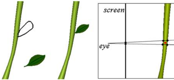
Fig. 10.19 When the stroke starts and ends over the active model (the stem) the depth of the active model in the vicinity of the stroke is used in the translation. Inset: the local depth (at the red point ) is computed by averaging the entry and exit points of two rays cast from the view point (eye), through the start and end of the stroke on the screen plane, and into the model
