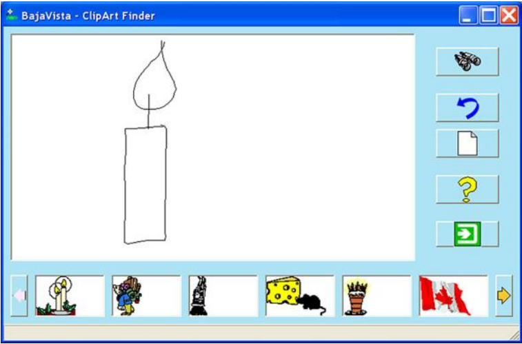
Fig. 7.15 First clip art finder prototype (BajaVista). Similar results to the sketch are presented at the bottom, the best candidate being the first on the left
