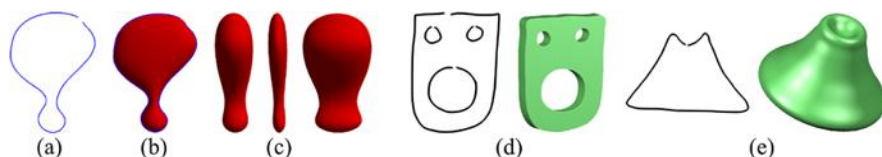
Fig. 11.8 Blobsy inflation converts the 2D sketch shown in a into the 3D volume b such that the 2D sketch lies on the 3D silhouette. The width of the inflated volume can be manipulated interactively, shown in (c) . Sketched 2D curves can also be used to create d linear sweeps and e surfaces of revolution
