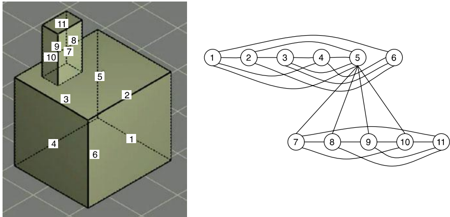
Fig. 7.18 3D object ( left ) and correspondent faces graph, used to compute the signature of the object
