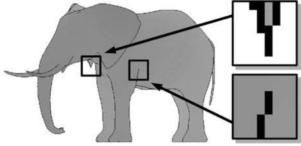
Fig. 9.23 Depth map with binary overlay from (11) (left), degenerated silhouette feature (top, right), silhouette caused by a surface crease (bottom, right)
