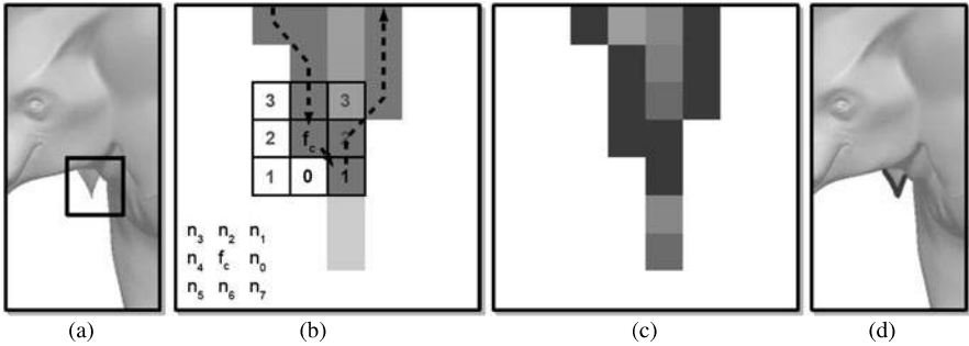
Fig. 9.24 Tracing the silhouette path near a degenerate feature (from left to right): a Elephant’s ear, b tracing step ( f_c \rightarrow n_7 ) with priority map, neighborhood index ( bottom left ) and a degenerate feature in light grey (which is removed in a pre-processing step), c final silhouette path ( dark pixels ), d extracted silhouette
