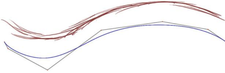
Fig. 13.2 B-spline fitting to raw strokes. Top: Input strokes. Bottom: Resulting B-spline and its control polygon
