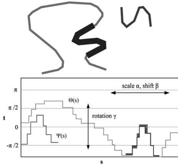
Fig. 9.26 Top : the short, medium grey target polyline, light grey silhouette, and best match (dark grey/thick) shown as a subset of the silhouette polyline. Bottom : arclength vs. cumulative turning angle representations of target \Psi(s) , silhouette \Theta(s) , and best-match polylines (bottom)
