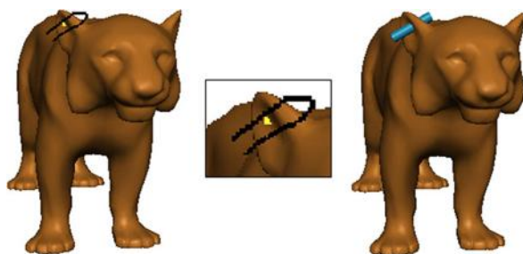
Fig. 10.21 An active point can be used when the center of the model does not provide an accurate enough depth. Here, the active point is on the left ear
