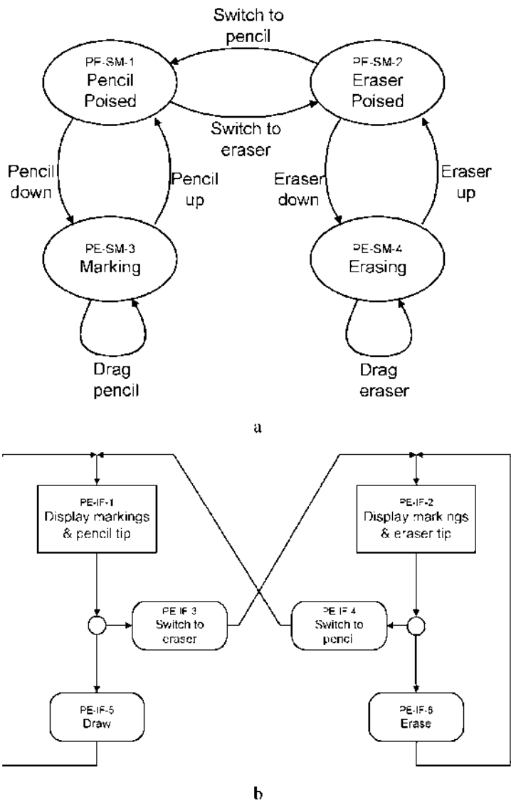
Fig. 3.6 a State Machine and b Interaction Flow diagram for pencil and eraser. Rectangles represent a quiescent state of the interface. Rounded rectangles represent user actions. Circles represent user choices among available actions, given the presentation state
