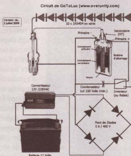
Ganga-Shakti circuit de GoToLuc.
